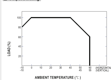
Output Derating
